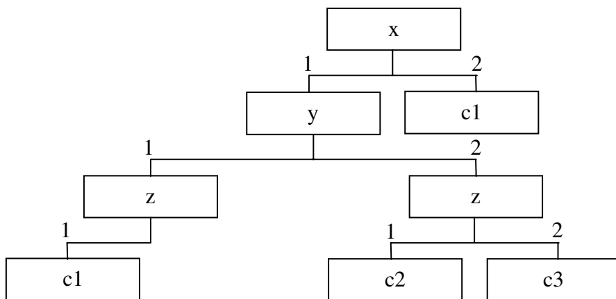
Figure 8.2 Decision Tree Generated from Figure 8.1 by ‘Delete Branch’ Strategy
